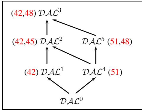
Figure 1. A lattice of \mathcal{DAL}^n systems
