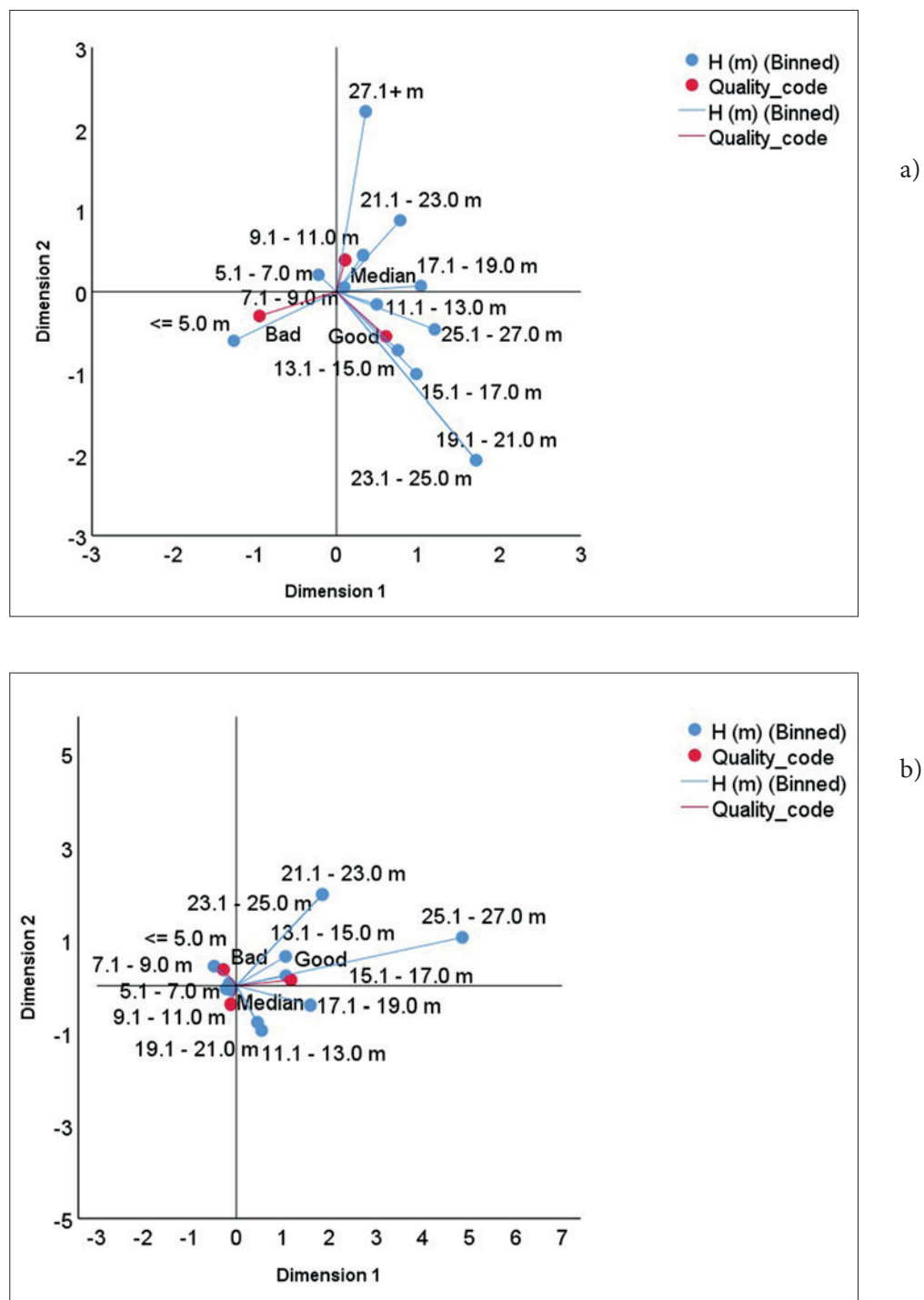
Figure 7. Association analysis between the height and the tree quality for a) Plot 1, and b) Plot 2
