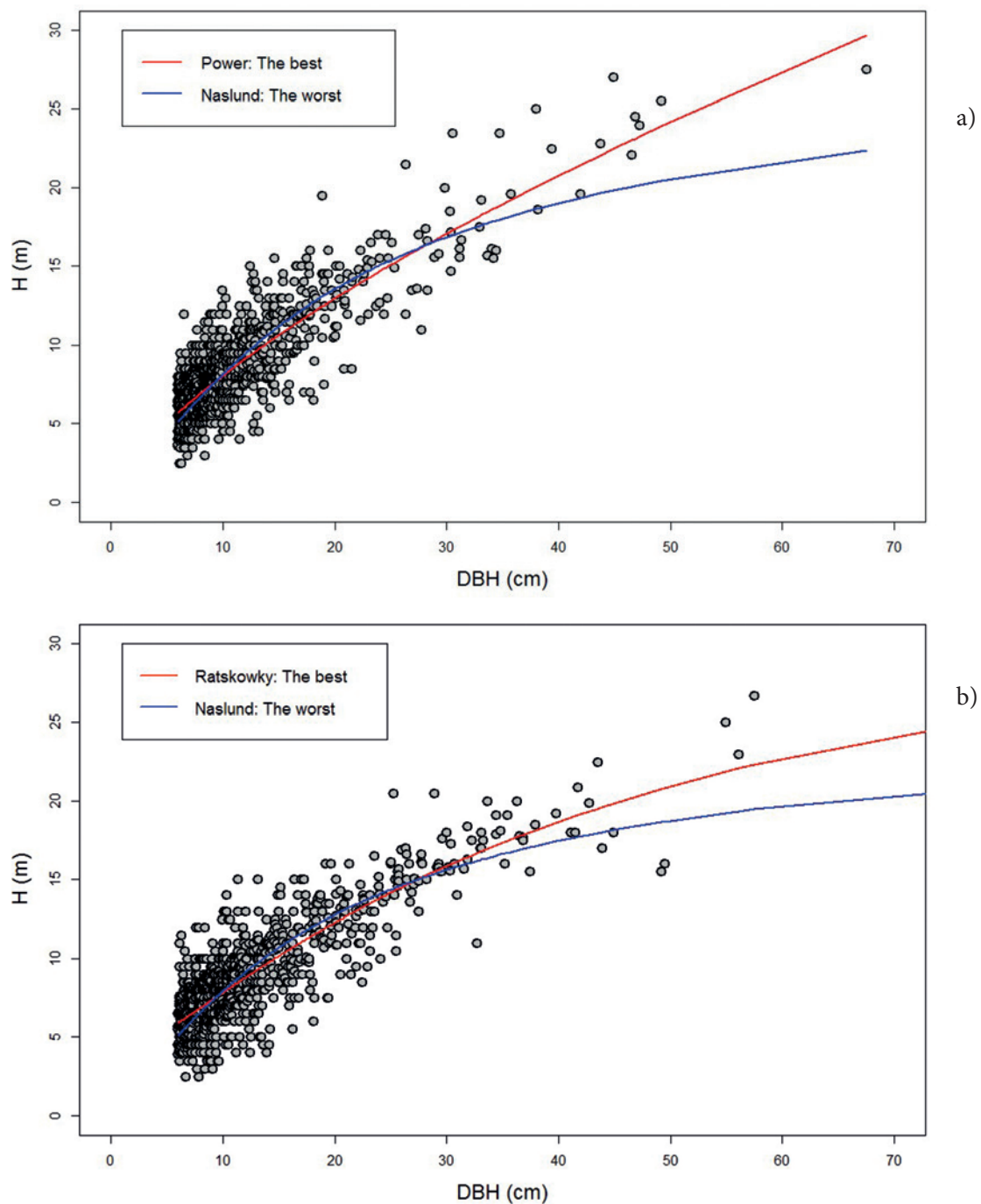
Figure 5. Regression charts for the best (red line) and the worst (blue line) models for a) Plot 1, and b) Plot 2
