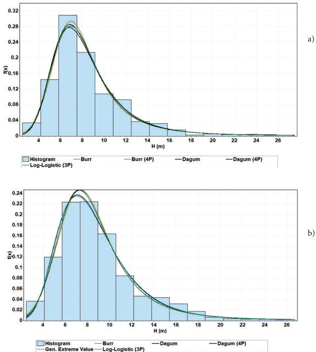
Figure 4. Five best fitted curves for the height variable a) for Plot 1; b) for Plot 2
