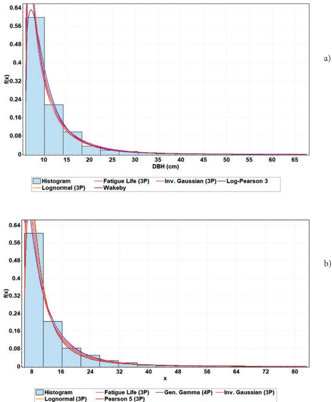
Figure 3. Five best fitted curves for the diameter variable a) for Plot 1; b) for Plot 2
