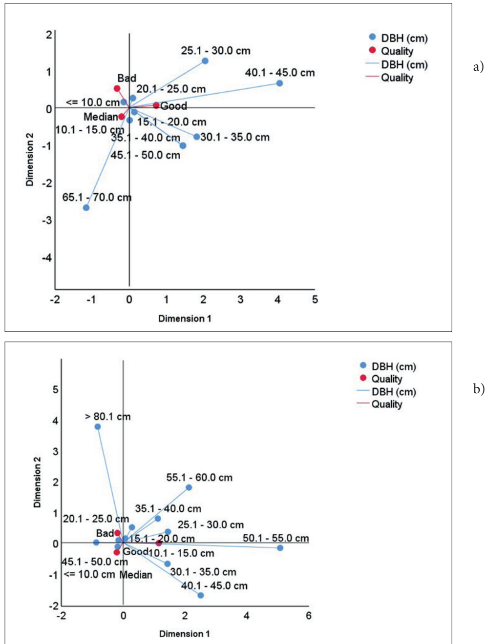
Figure 6. Association analysis between the diameter and the tree quality for a) Plot 1, and b) Plot 2
