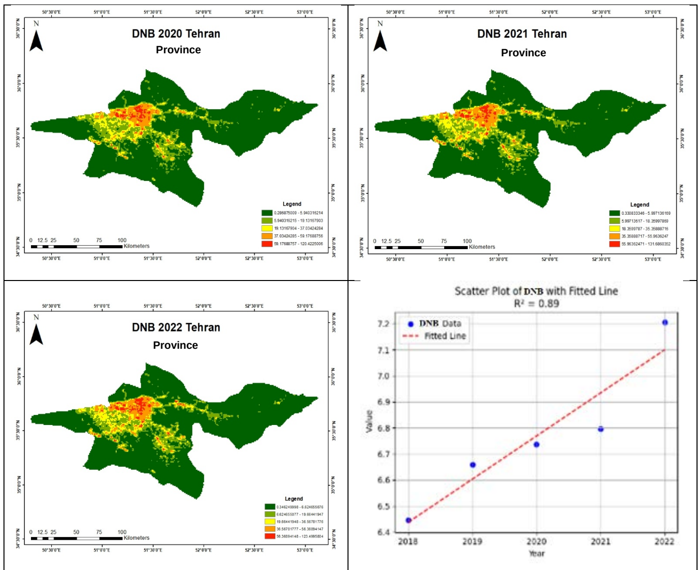
Figure 2. Source: VIIRS DNB, NASA, 2018–2022. Spatial distribution and annual trend of DNB value (nanoWatts/sr/cm 2 ) in Tehran Province
