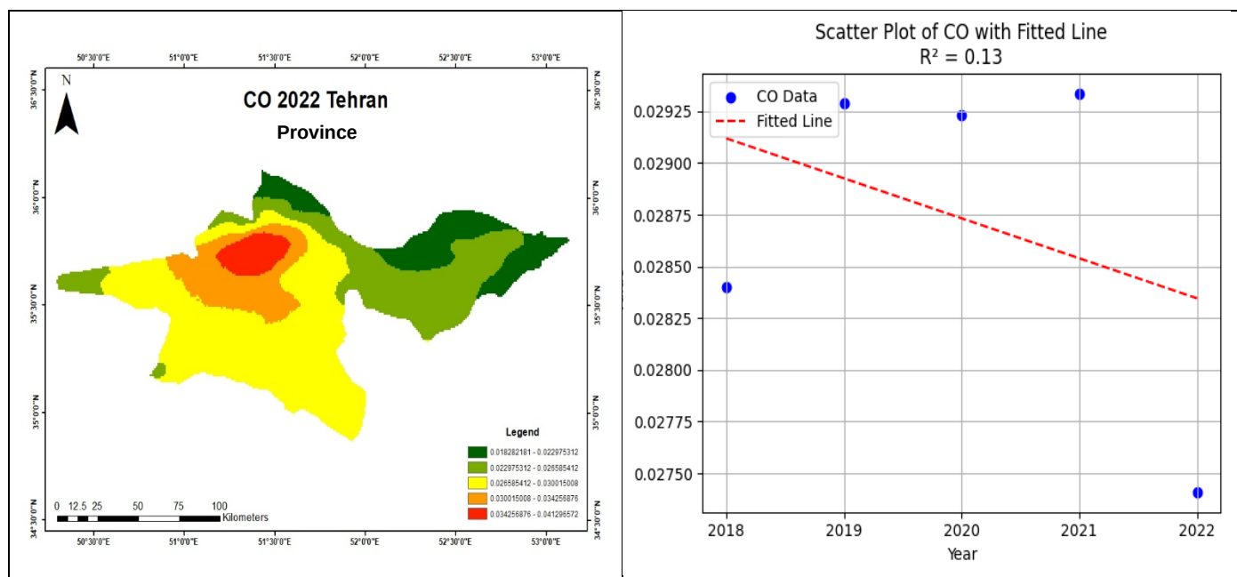
Figure 4. Source: CO, ESA sentinel, 2018–2022. Spatial distribution and annual trend of CO values (mol/m 2 ) in Tehran Province
