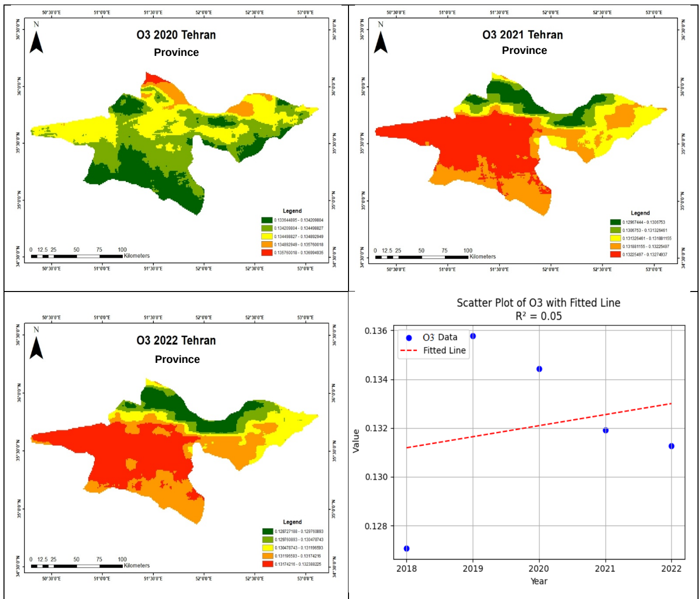
Figure 5. Source: O 3 , ESA sentinel, 2018–2022. Spatial distribution and annual trend of O 3 values (mol/m 2 ) in Tehran Province
