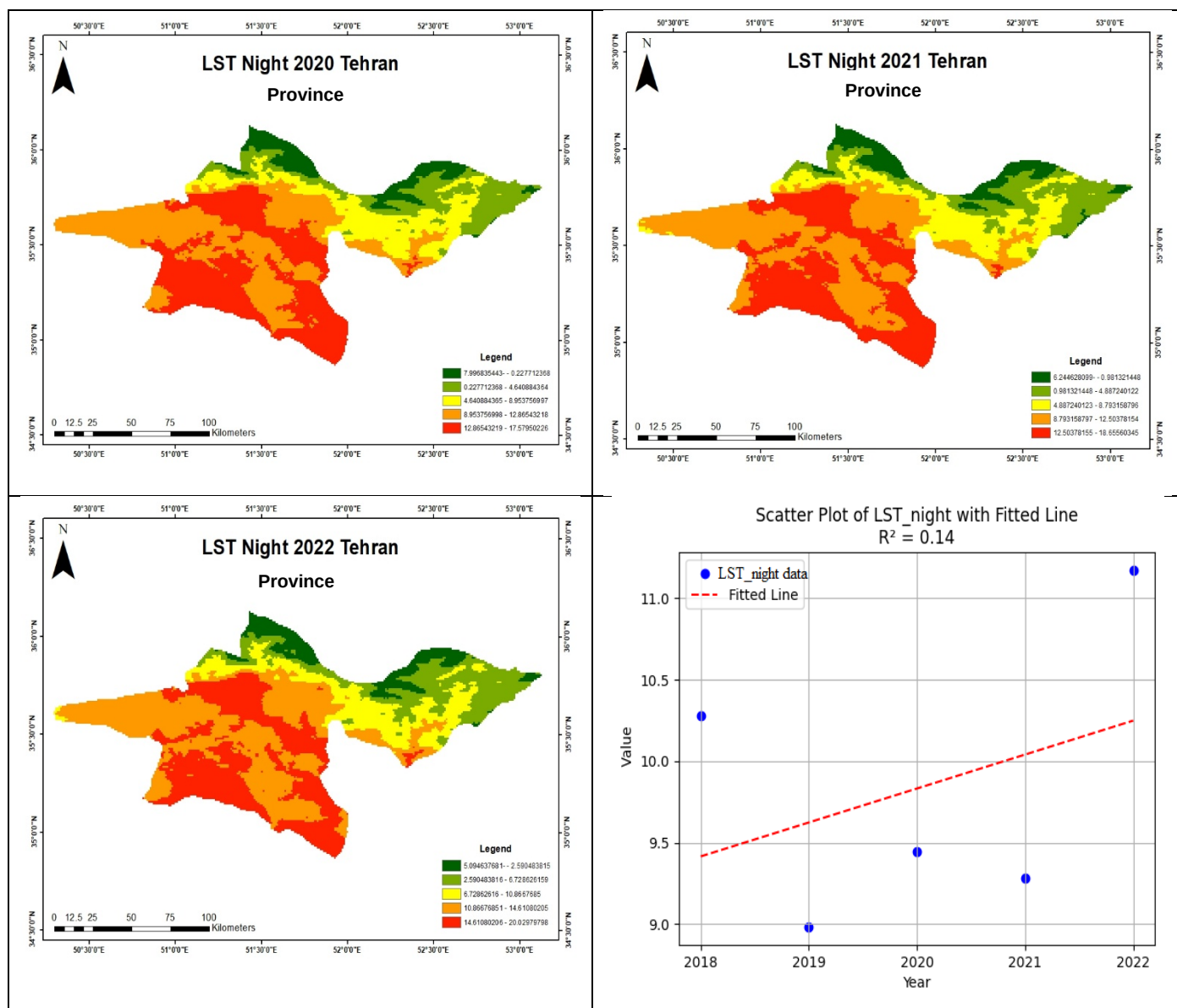
Figure 7. Source: LST_night, NASA, 2018–2022. Spatial distribution and annual trend of LST_night values (°C) in Tehran Province
