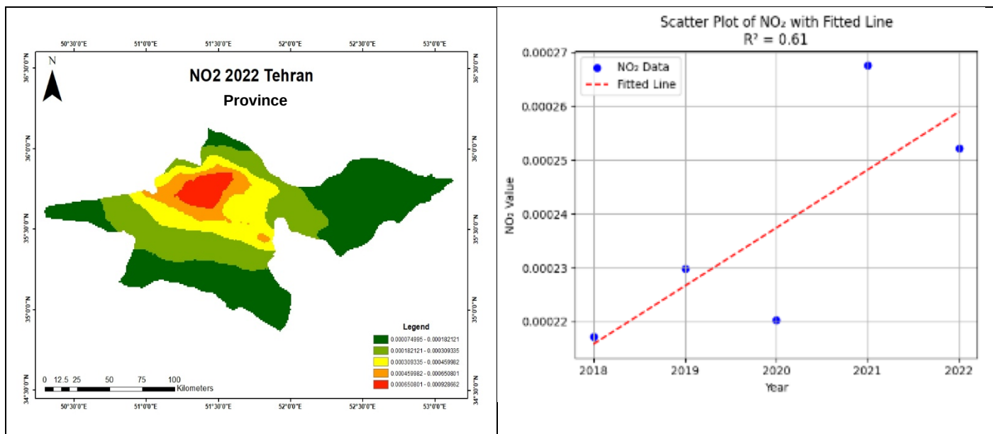
Figure 3. Source: NO 2 , ESA sentinel, 2018–2022. Spatial distribution and annual trend of NO 2 values (mol/m 2 ) in Tehran Province
