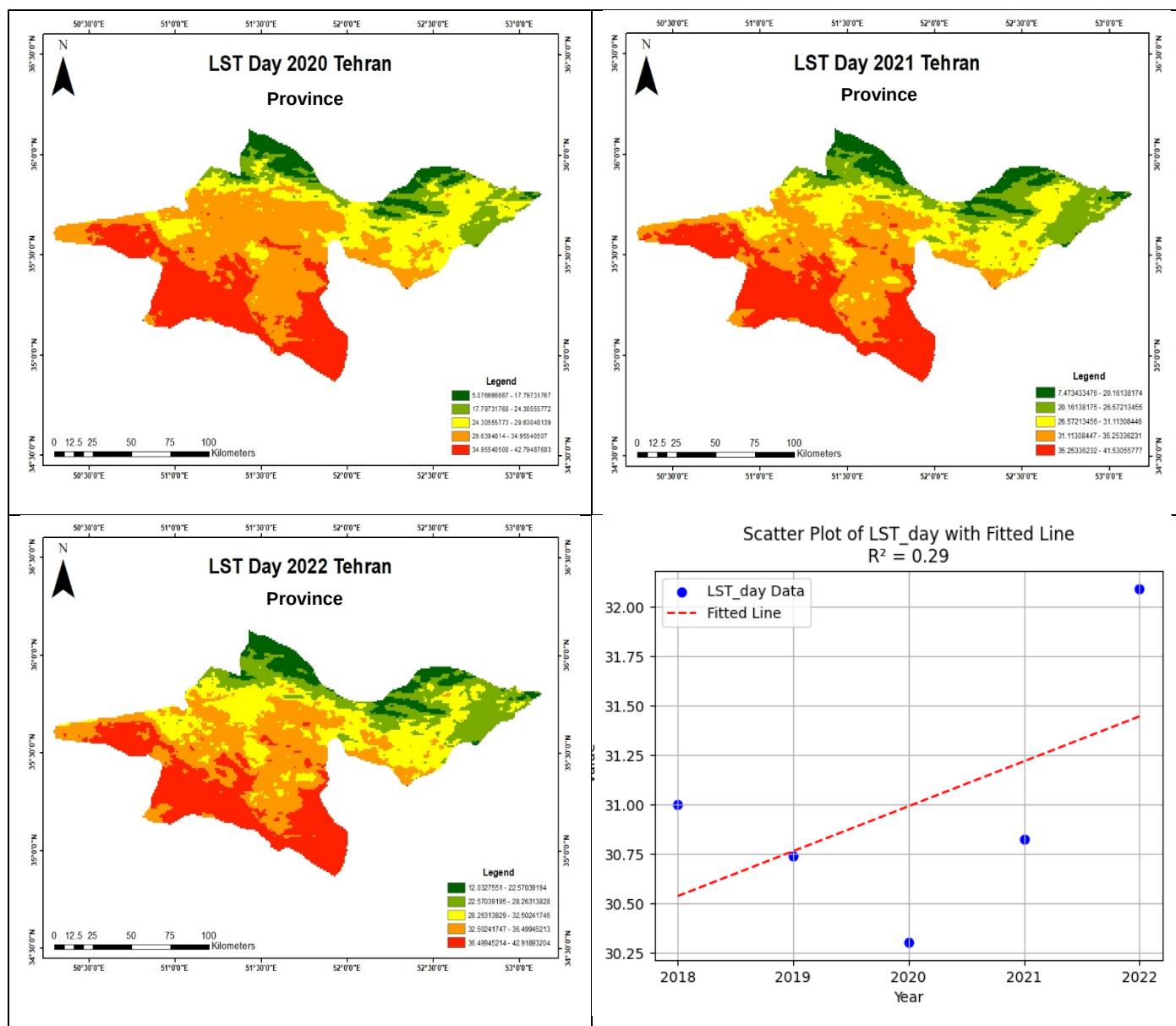
Figure 6. Source: LST_day, NASA, 2018–2022. Spatial distribution and annual trend of LST_day values (°C) in Tehran Province
