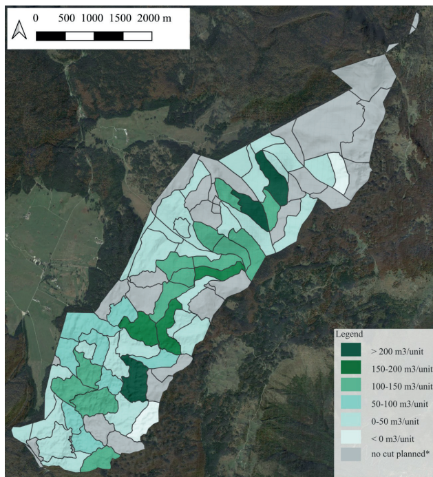
Figure 4. Map of timber provision value of the Cansiglio Orientale forest. *in grey, the units where no timber cutting is foreseen in the period considered (classes of 50 \text{ m}^3/\text{unit} )
