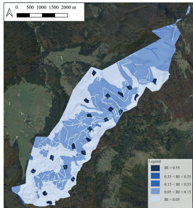
Figure 7. Map of the biodiversity value of the Consiglio Orientale forest divided in classes within a range between 0 (minimum value) and 1 (maximum value). The biodiversity indicator (BI) is dimensionless
