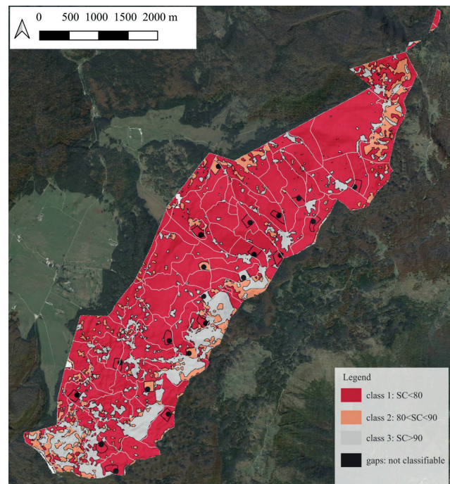
Figure 5. Stand stability map of the Cansiglio Orientale forest by classes (high stand stability in red; medium stand stability in orange; low stand stability in grey; gaps where all the trees have been cut down in black) after the realisation of the SHSs
