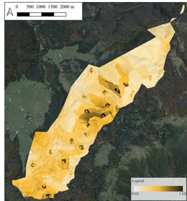
Figure 8. Map of the aggregated value of the ecosystem services provided by Cansiglio Orientale forest. The ES global indicator (GI) is dimensionless
