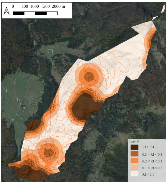
Figure 6. Map of the recreational value of the Consiglio Orientale forest by classes within a range between 0 (minimum value) and 1 (maximum value). The recreational indicator (RI) is dimensionless
