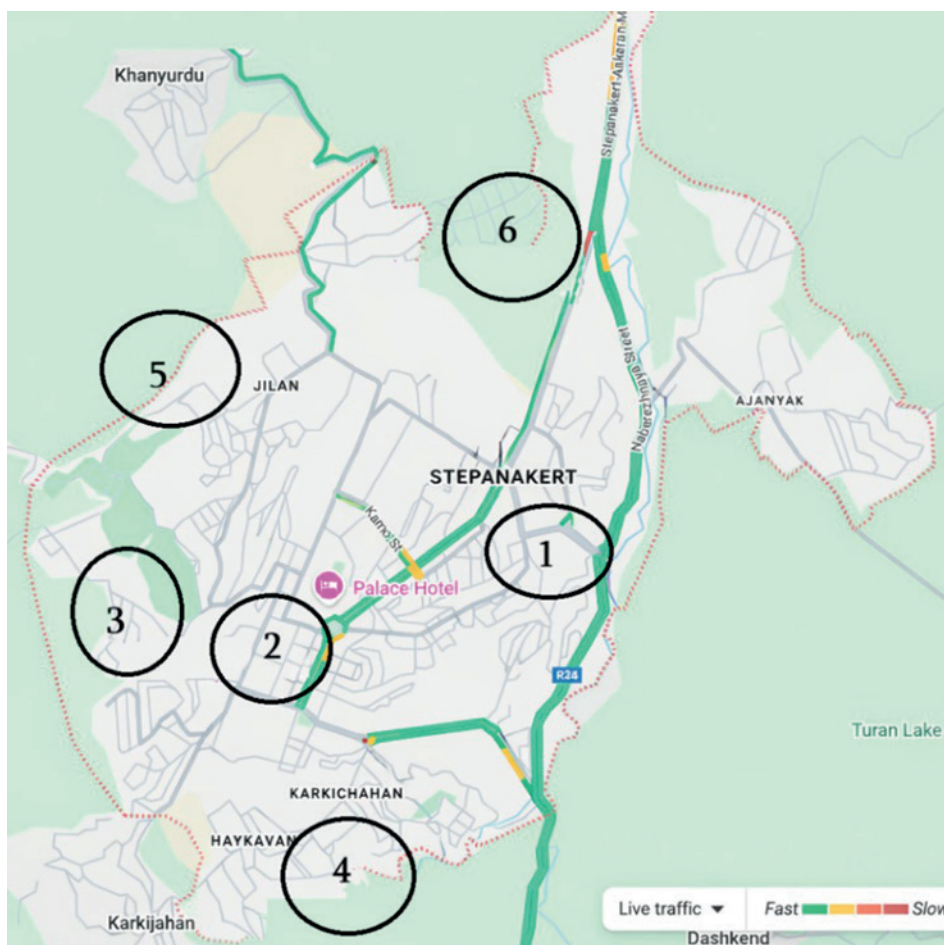
Figure 1. Map of stationary monitoring stations 1. Grove, 2. Park, 3. Cemeteries, 4. Orchard, 5. Bushes, 6. Urban Forest
