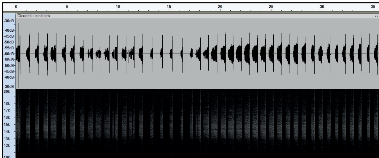
Figure 5. Oscillogram (above) and spectrogram (below) of a 36-second recording of calling song of C. cantilatrix , Kalina-Lisiniec Natura 2000 site PLH120007, 21 V 2024. Sound recorded with Tascam DR-07X audio recorder without external microphone, in PCM 44,1 kHz stereo (for clarity only one of the two audio channels is presented)
