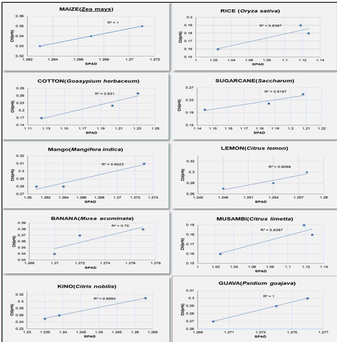
Figure 2. Relationship of total Chl(a+b) and SPAD
