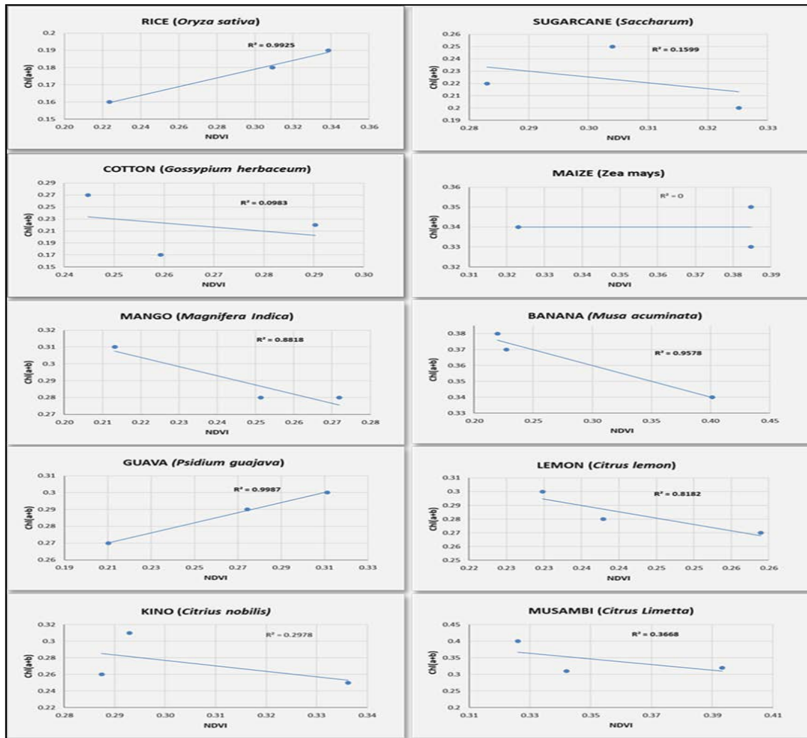
Figure 4. Relationship among NDVI and Chl (a+b)
