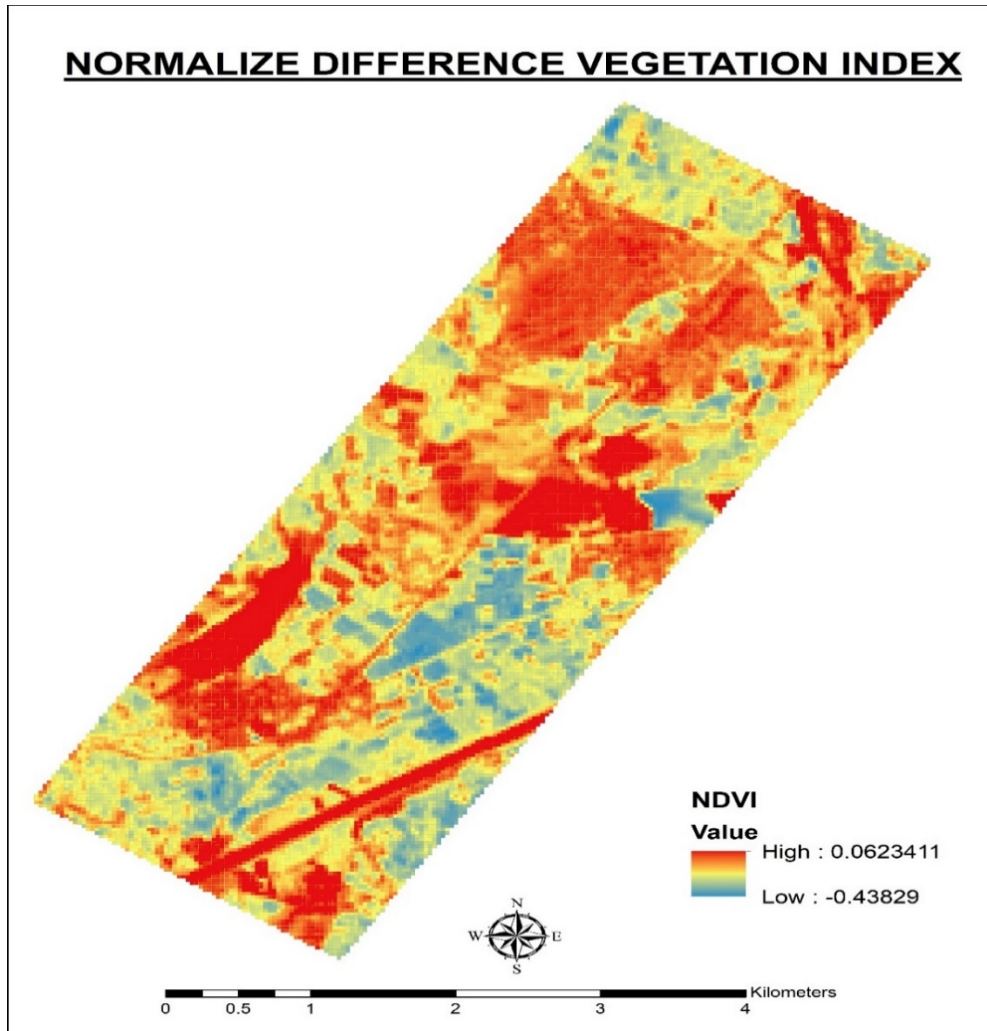
Figure 2. Normalize difference vegetation index
