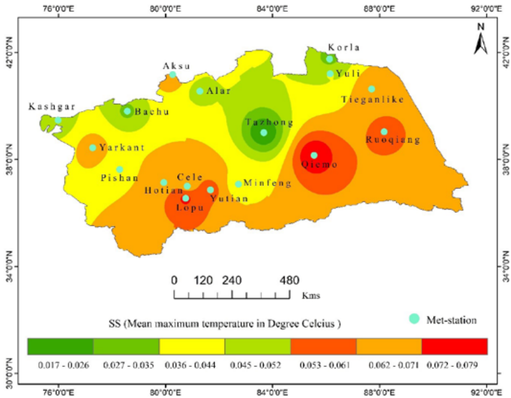
Figure 5. Sen's slope values Interpolation of mean monthly maximum temperature
