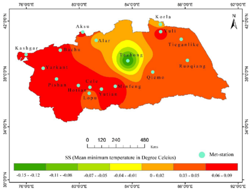
Figure 6. Interpolation of Sen's slope values mean monthly minimum temperature
