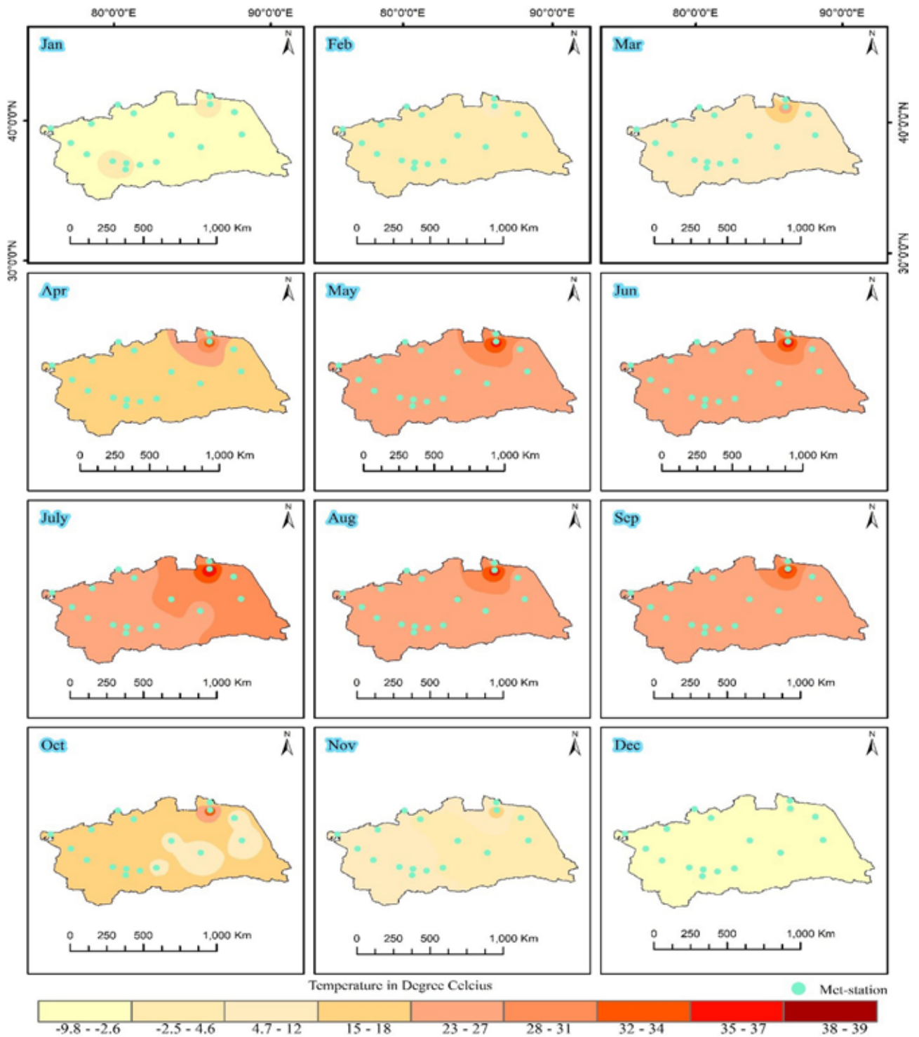
Figure 3. Maps shows mean monthly temperature interpolation (1 to 12 months) in selected met-stations
