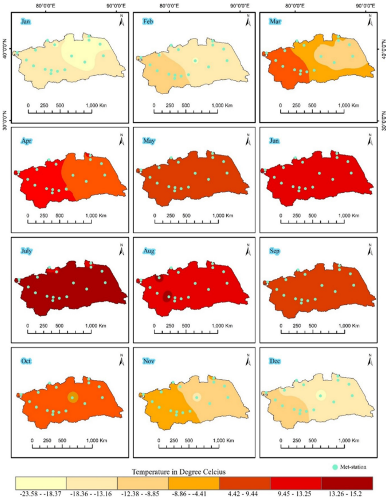
Figure 4. Maps shows interpolation of mean monthly minimum temperature (1 to 12 months) of selected met-stations
