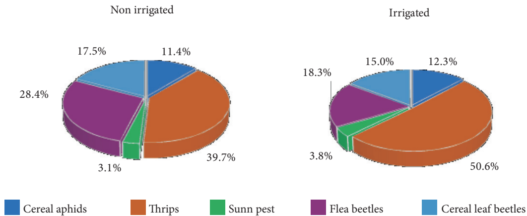
Figure 1. The structure of the main phytophagous complex of winter wheat depending on irrigation (2015-2020)
