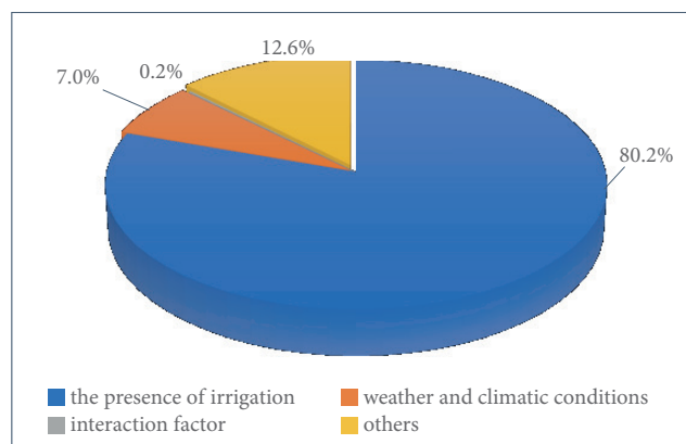
Figure 2. The influence of the studied factors on the number of Sunn pest on winter wheat crops
