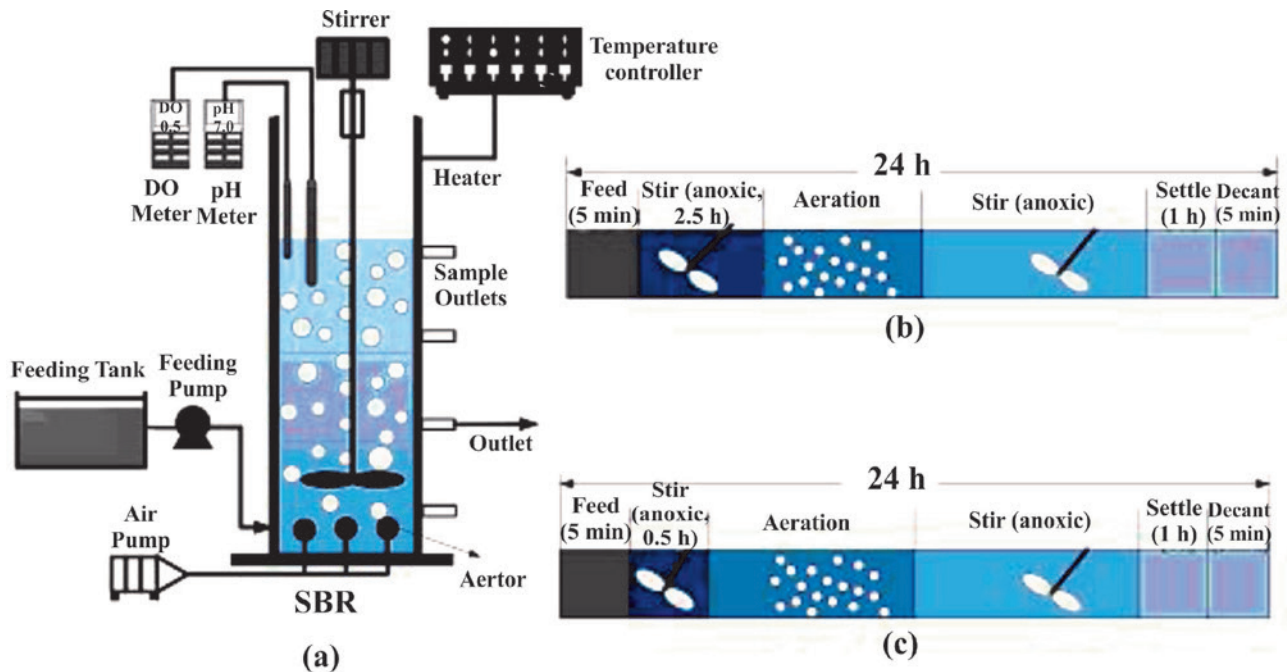
Figure 1. The various modes of operation for an SBR system: (a) Innovative schematic diagram of modified SBR (b) operational steps with three phase cycle and (c) operational steps of the modified SBR with four cycles (Miao et al., 2015a)
