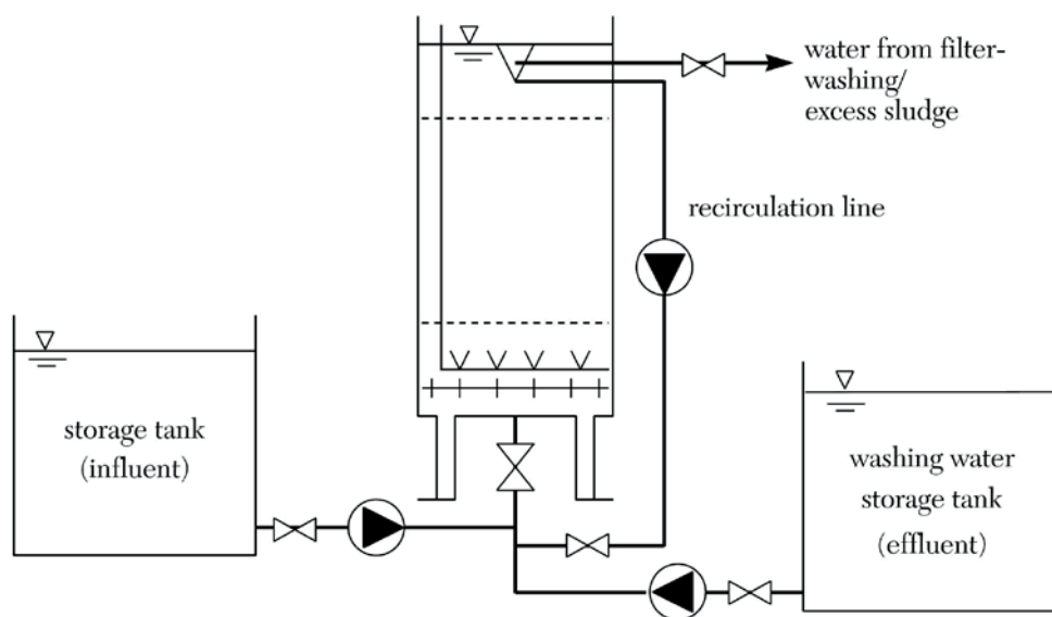
Figure 2. Schematic over view of an modified upflow SBBR (National & Pillars, 2015)
