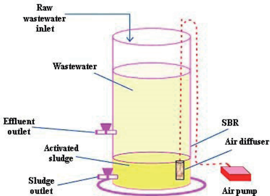
Figure 3. Typical cylindrical type SBR (Su et al., 2018)
