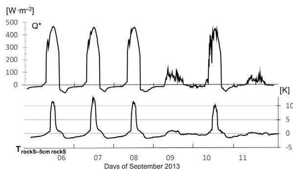
Fig. 5. Daily course of the net radiation ( Q^* ) at the bottom of the canyon and the temperature differences \Delta T_{\text{rockS-5cm rockS}} = T_{\text{rockS}} - T_{\text{5cm rockS}} at Rękawica complex in the period of 5–11.09.2013
