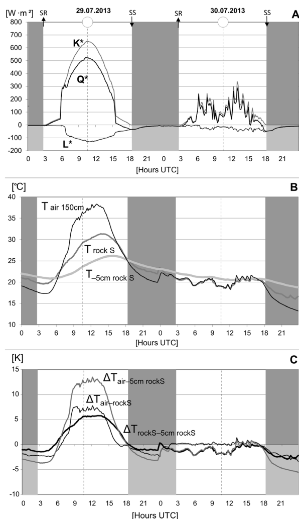
Fig. 2. Variation of: (A) the radiation balance elements; (B) the temperature of the air and rock; (C) temperature differences T_{\text{air}} - T_{\text{rock S}} ( \Delta T_{\text{air-rock S}} ), T_{\text{air}} - T_{\text{5cm rock S}} ( \Delta T_{\text{air-5cm rock S}} ), T_{\text{rock S}} - T_{\text{5cm rock S}} ( \Delta T_{\text{rock S-5cm rock S}} ) at the bottom of the canyon in Ojców on 29–30.07.2013
