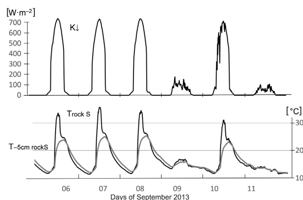
Fig. 4. Daily course of the global radiation ( K\downarrow ), temperature of the rock S: on the surface ( T_{\text{rockS}} ) and at the depth of -5\text{ cm} in the rock ( T_{-5\text{cm rockS}} ) at Rekawica complex in the period of 5–11.09.2013
