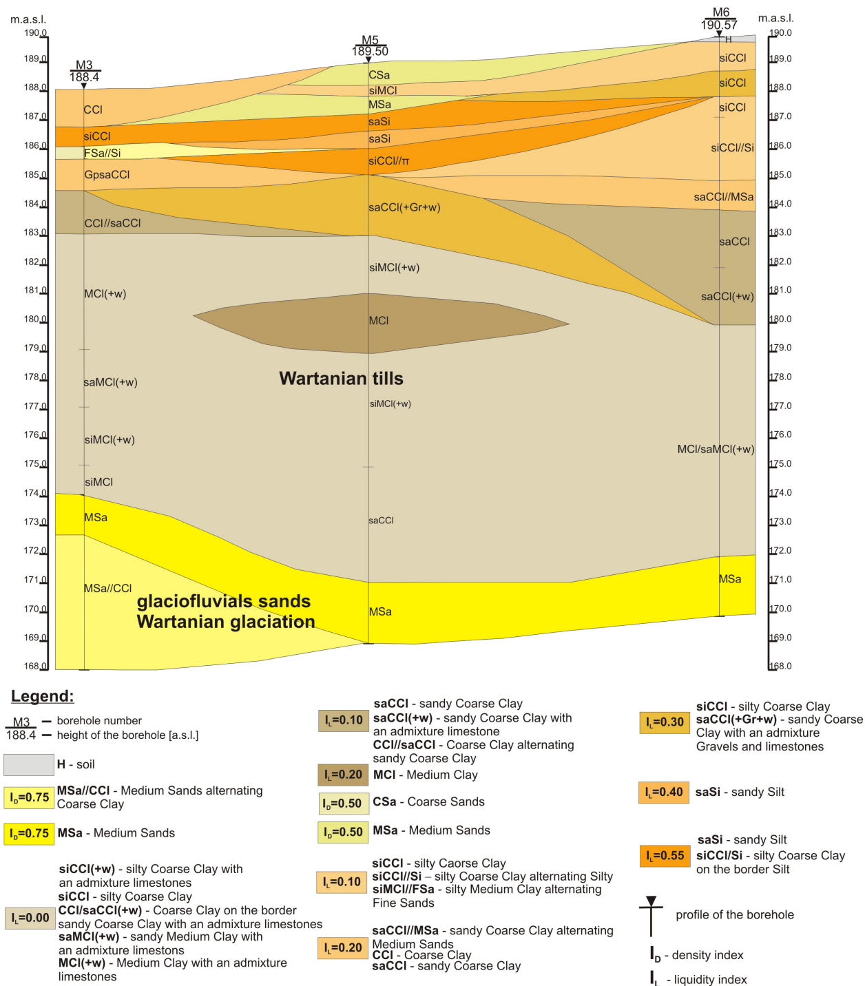
Fig. 2. Synthetic geological cross-section in Pabianice (based on the card of boreholes according to Libera et al. 2008)
