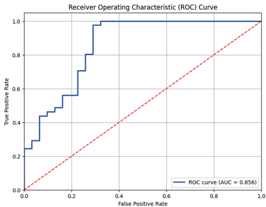
Fig. S3. ROC curve of the SVM model, simulated using the CHIRPS rainfall dataset as part of the entire set of factors
