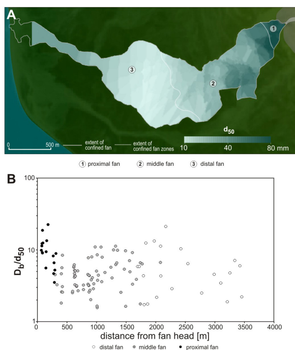
Fig. 7. Grain size-distribution characterised by spatial and downfan changes in median grain diameter (A) and downfan changes of D_b/d_{50} index (B)
