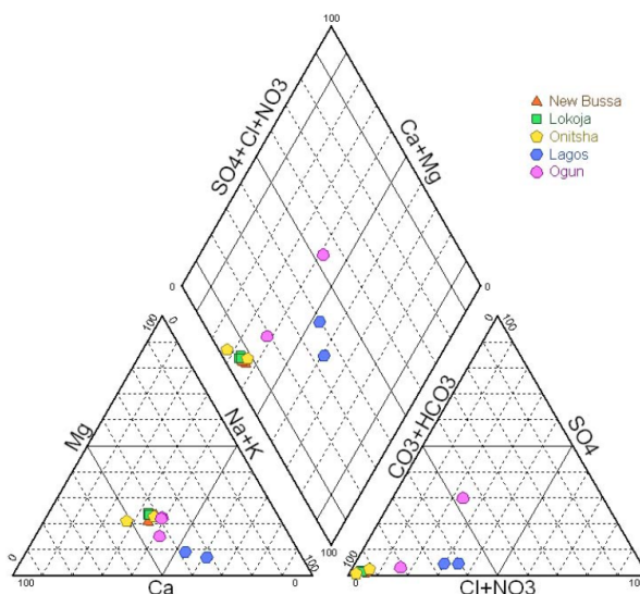
Fig. 5 Piper diagram of sampled water of lower Niger River basin and part of the Lagos region (Nigeria)
