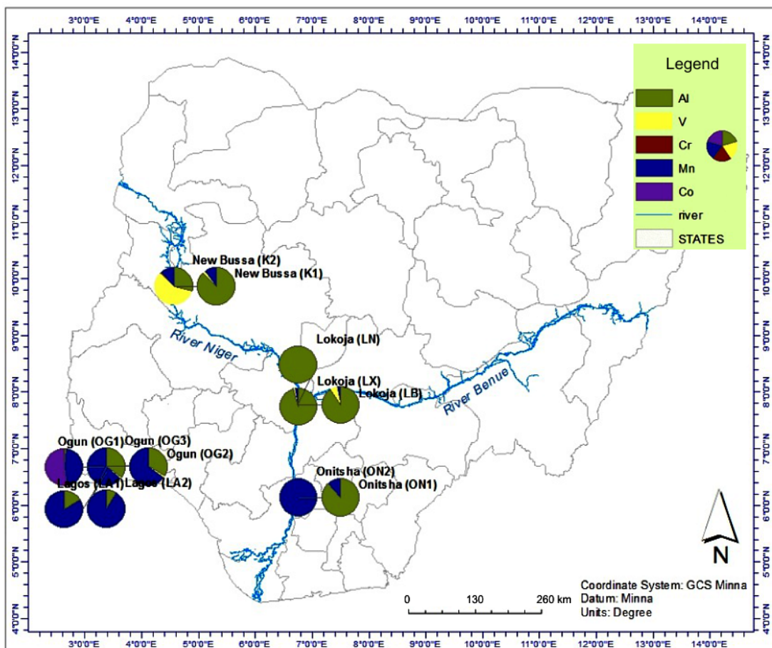
Figure 4. Selected trace element distributions in sampled water stations
