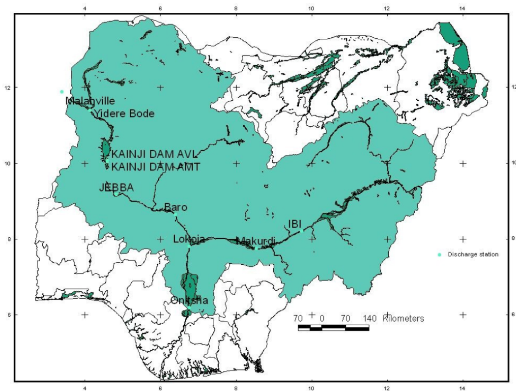
Fig. 1: Lower Niger River basin - position of the sample stations show on the map
